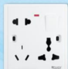
Combination Socket with Switch 13A, 250V 901689
