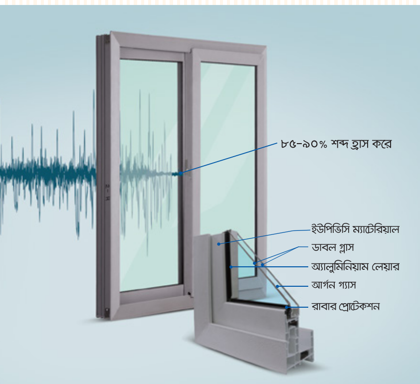
EMBOSS DOUBLE GLAZING WINDOW
